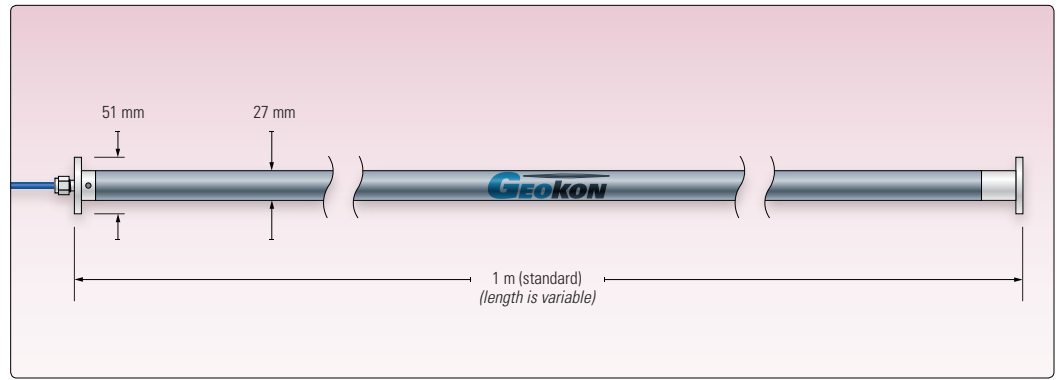
• Model 4430 dimensions.
